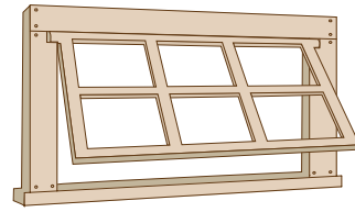
W114NEB WORK CAR WINDOW 12/BAG - W/GLAZING 18"W x 28"H .26" x .37" Opening
