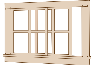
W109NEB 4/4 DBL HUNG WINDOW 8/BAG - W/GLAZING 52"W x 42"H .65" x .53" Opening
